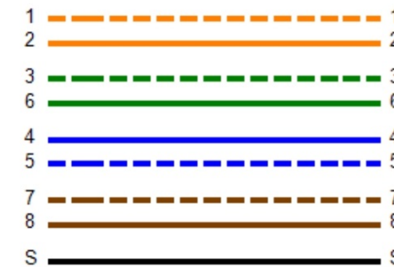
Wire Map (T568B) PASS
